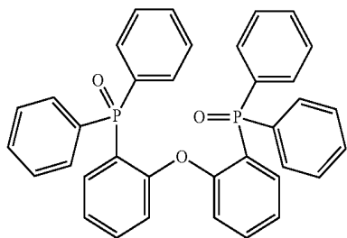
[Chemical Formula 76]
