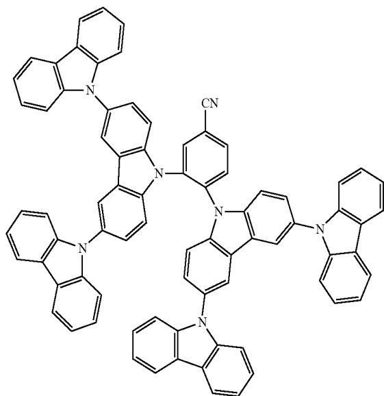
[Chemical Formula 44]
