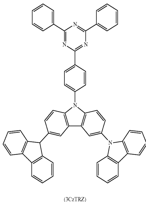
[Chemical Formula 91]
