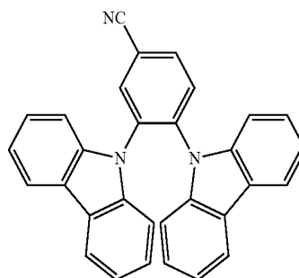
[Chemical Formula 87]
