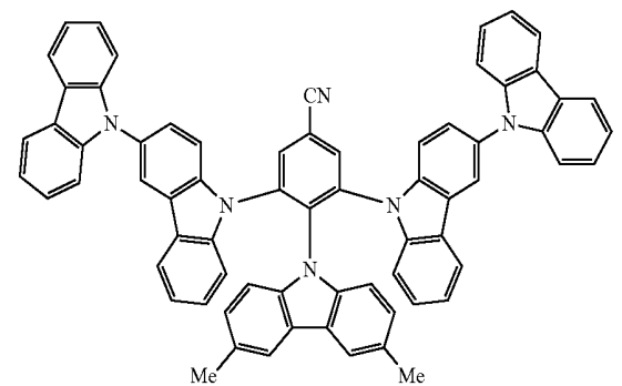
[Chemical Formula 45]
