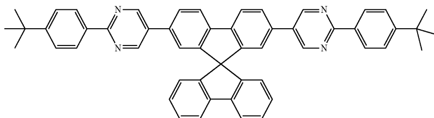
[Chemical Formula 62]
