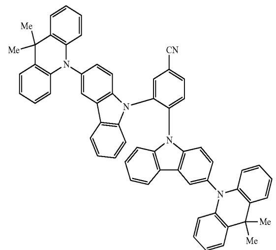
(Compound 41)
