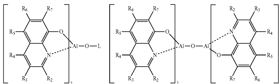
[Chemical Formula 63]
