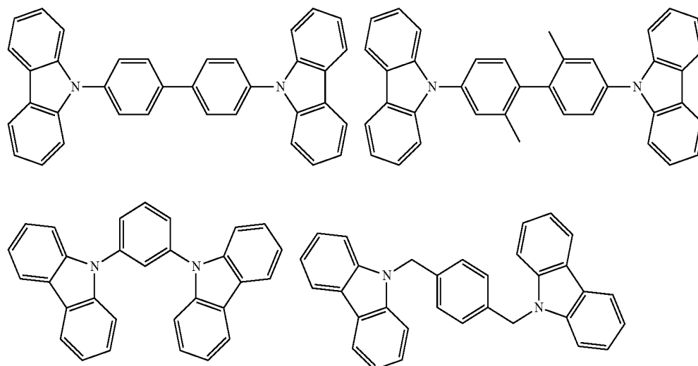
[Chemical Formula 63]
