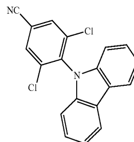
[Chemical Formula 8]
