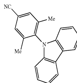
[Chemical Formula 6]
