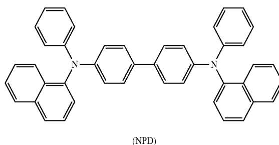
[Chemical Formula 93]
