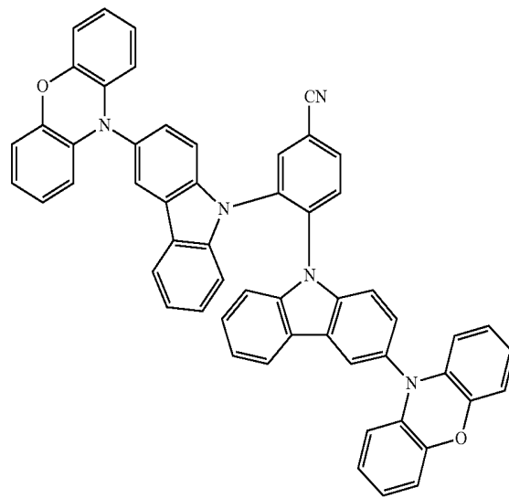
(Compound 42)
