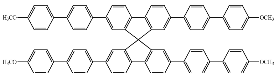
[Chemical Formula 61]
