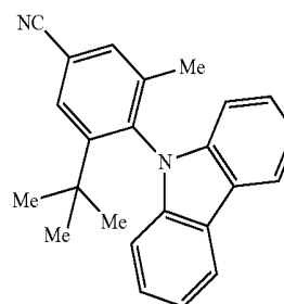
[Chemical Formula 7]
