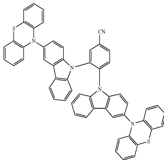
(Compound 43)
