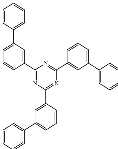
(T2T)
